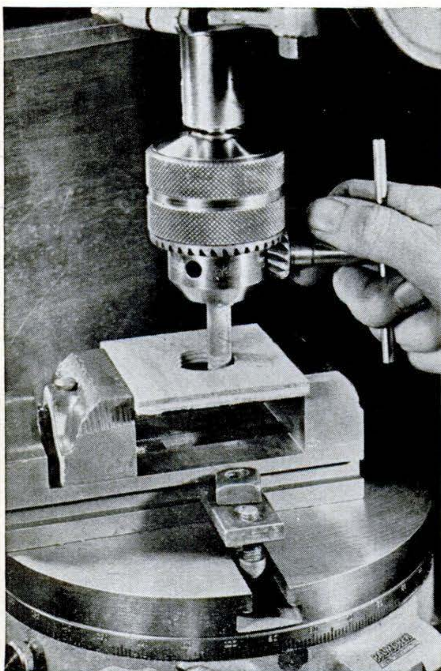
USING ROTARY FEED, a hole in a lens board is sanded with a small spindle. Unless hole was bored at same setup, be careful to locate it over the center of rotary table.
